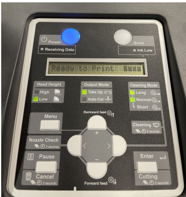
Mutoh XpertJet 1341SR Pro control panel
